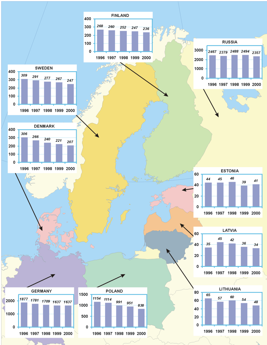
Figure 4.5 Map of annual emissions of nitrogen oxides from individual HELCOM countries in the period 1996 – 2000. Units: ktonnes/yr.
