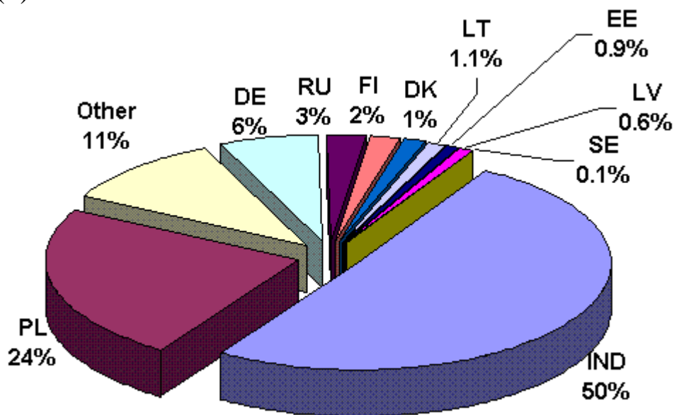
Figure 4.15 Comparison of main emissions sources of cadmium contributing to its annual deposition over the entire Baltic Sea Basin 1996 (a) and 2000 (b). Other – means other European countries in total, IND – means indeterminate sources: natural, previous and remote anthropogenic sources.
