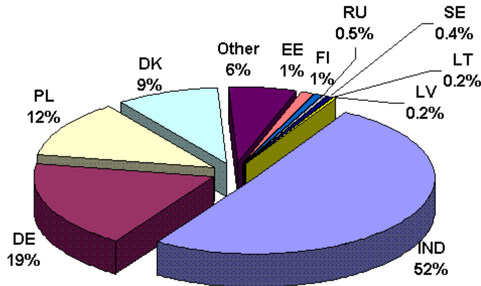
Figure 4.17 Comparison of main emissions sources of mercury contributing to its annual deposition over the entire Baltic Sea Basin in 1996 (a) and 2000 (b). Other – means other European countries in total, IND – means indeterminate sources: natural, previous and remote anthropogenic sources.
