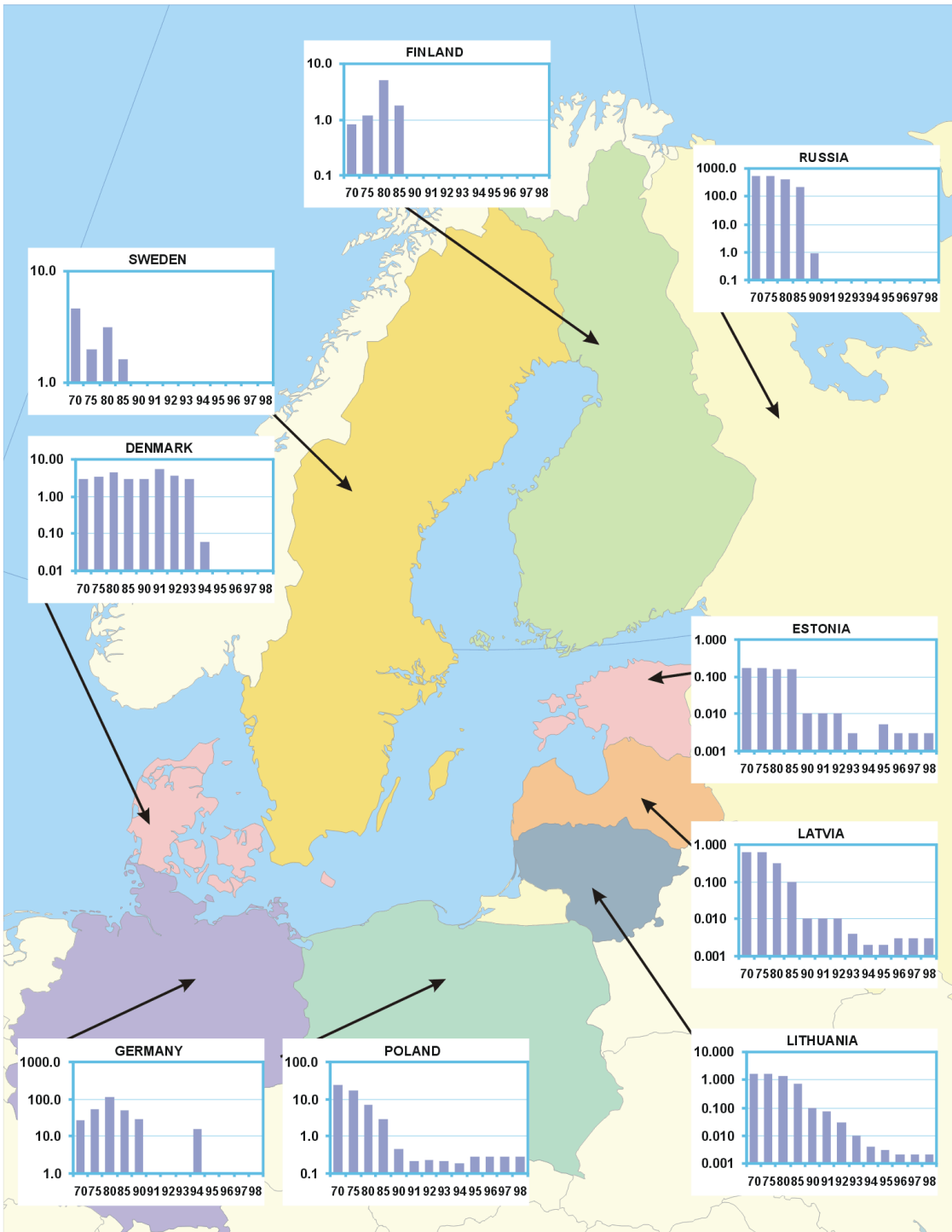
Figure 4.12 Map of annual total emissions of lindane from individual HELCOM countries in the period 1970 – 1998. Emission values are presented in the logarithmic scale. Missing bars correspond to lack of lindane emissions in particular year. Units: tonnes/yr.
