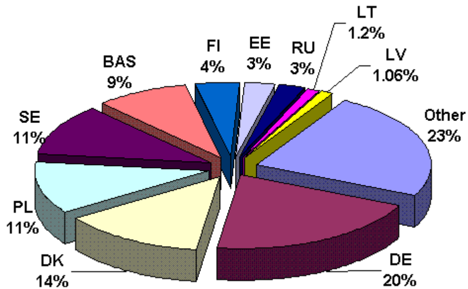
Figure 4.14 Main emissions sources of nitrogen contributing to its annual deposition over the entire Baltic Sea Basin in 1997.
