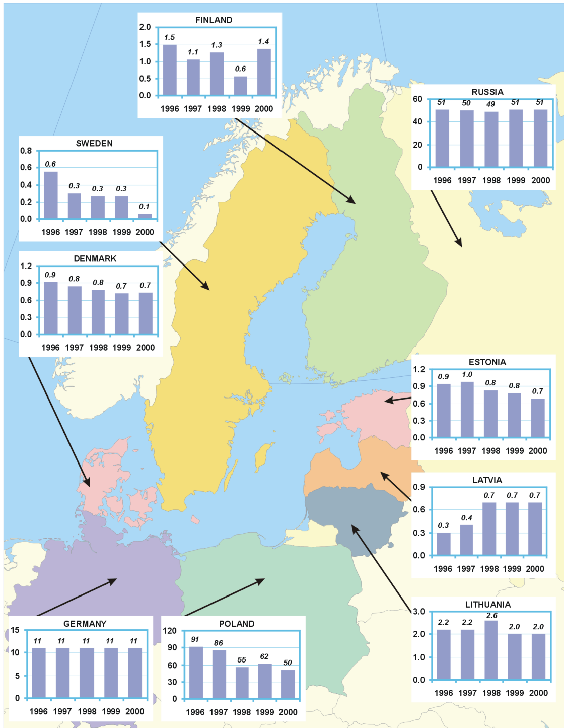
Figure 4.8 Map of annual emissions of cadmium from individual HELCOM countries in the period 1996 – 2000. Units: tonnes/yr.
