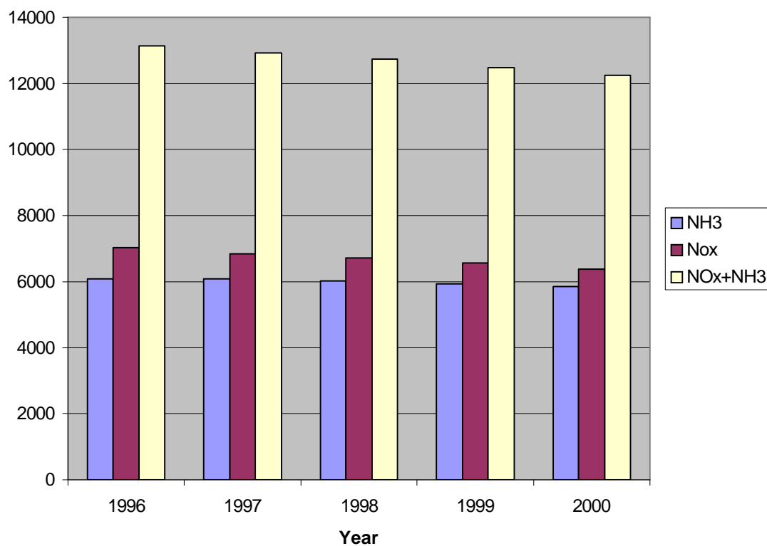
Figure 4.1. Annual emissions of nitrogen oxides, ammonia and total nitrogen (nitrogen oxides + ammonia) from the EMEP domain in the period 1996 - 2000. Units: ktonnes N/yr.
