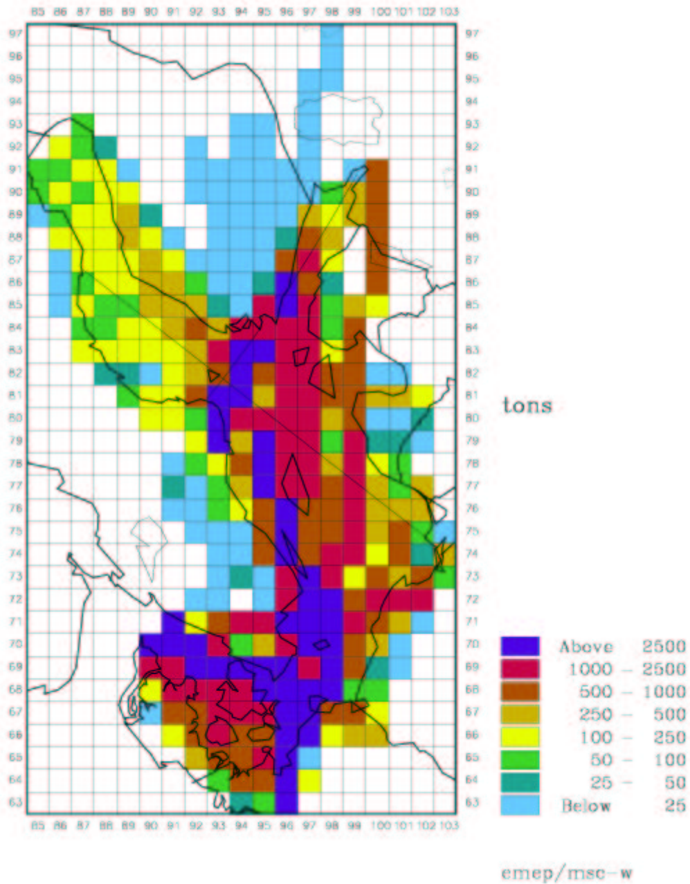
Figure 4.4 Map of annual emissions of nitrogen oxides from the international ship traffic on the Baltic Sea in 1990. Units: tonnes/yr/grid
