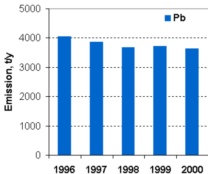
Figure 4.11 Annual emissions of cadmium, mercury and lead from all HELCOM countries in the period 1996 – 2000. Units: tonnes/yr.
