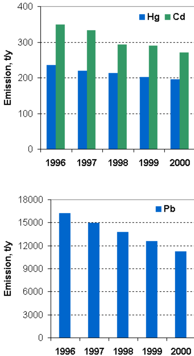
Figure 4.2. Annual emissions of cadmium, mercury and lead from the EMEP domain in the period 1996 - 2000. Units: tonnes /yr.
