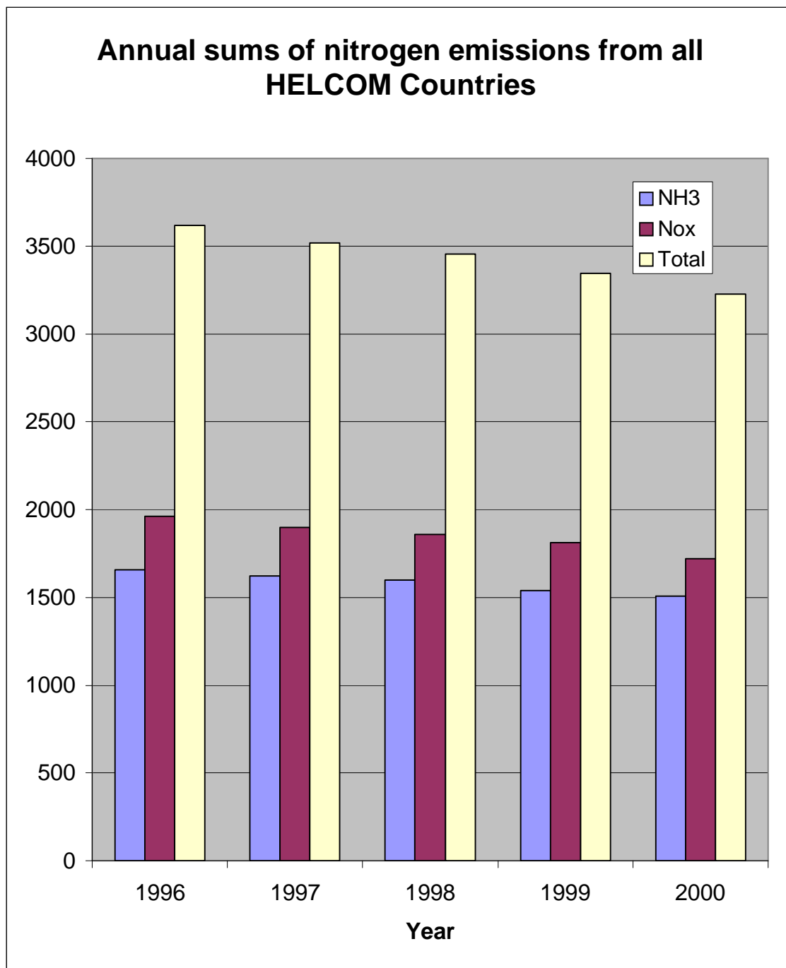
Figure 4.7 Annual emissions of nitrogen oxides, ammonia and total nitrogen (nitrogen oxides plus ammonia) from all HELCOM countries in the period 1996 – 2000. Units: ktonnes N/yr.
