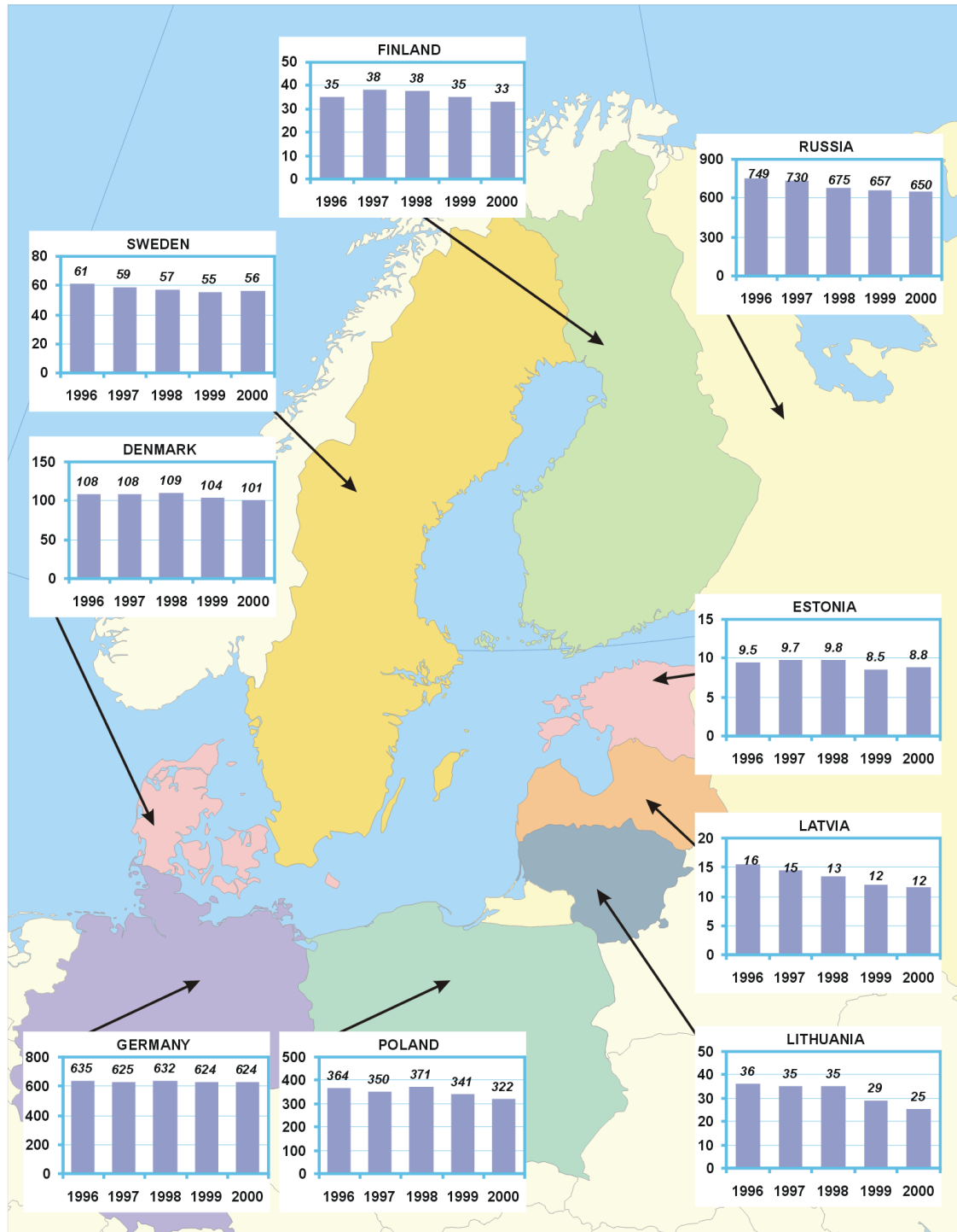
Figure 4.6 Map of annual emissions of ammonia from the HELCOM countries in the period 1996 – 2000. Units: kt/yr.
