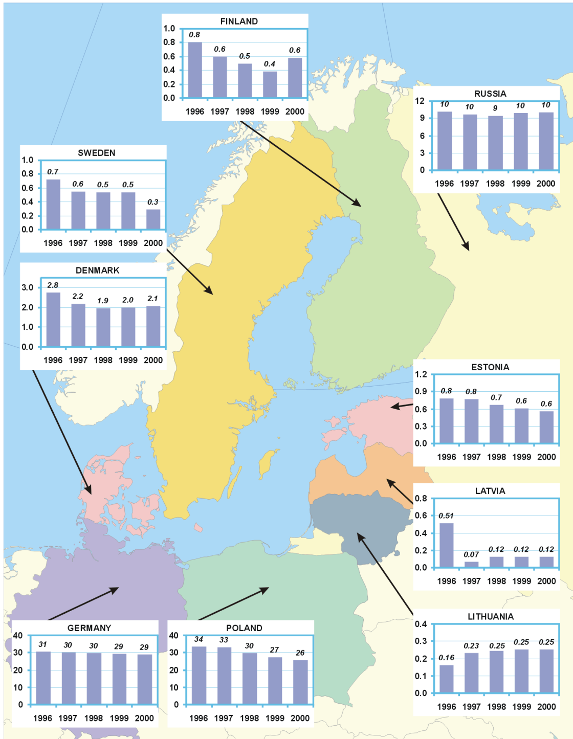
Figure 4.10 Map of annual total emissions of mercury from individual HELCOM countries in the period 1996 – 2000. Units: tonnes/yr
