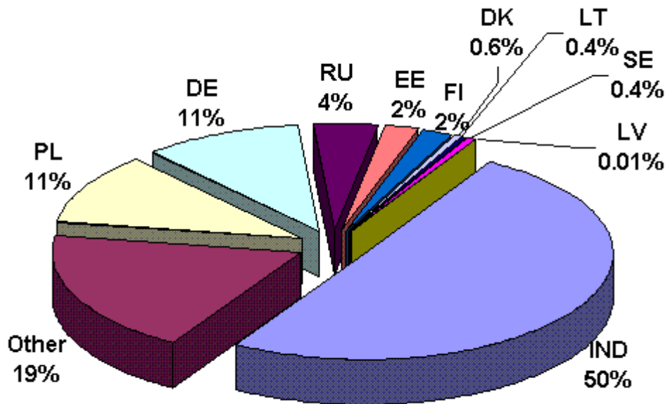
Figure 4.16 Comparison of main emissions sources of lead contributing to its annual deposition over the entire Baltic Sea Basin in 1996 (a) and 2000 (b). Other – means other European countries in total, IND – means indeterminate sources: natural, previous and remote anthropogenic sources.
