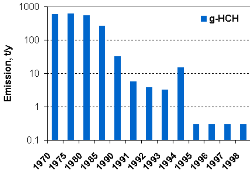
Figure 4.13 Annual total emissions of lindane from all HELCOM countries in the period 1970 – 1998. Emission values are presented in the logarithmic scale. Units: tonnes/yr.
