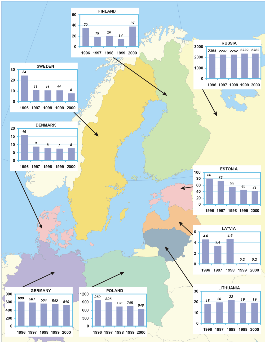
Figure 4.9 Map of annual total emissions of lead from individual HELCOM countries in the period 1996 – 2000. Units: tonnes/yr.
