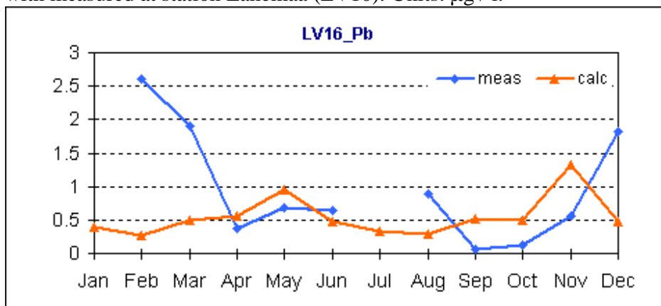
Figure 5.20. Comparison of calculated mean monthly lead concentrations in precipitation with measured at station Zoseni (LV16). Units: \mu\text{g} / \text{l} .
