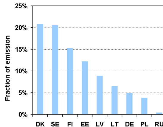
Figure 5.2. Fractions of lead anthropogenic emissions of HELCOM countries in 2002 deposited to the Baltic Sea.
