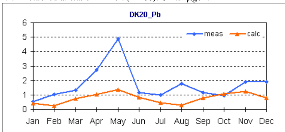
Figure 5.17. Comparison of calculated mean monthly lead concentrations in precipitation with measured at station Pedersker (DK20). Units: \mu\text{g} / \text{l} .
