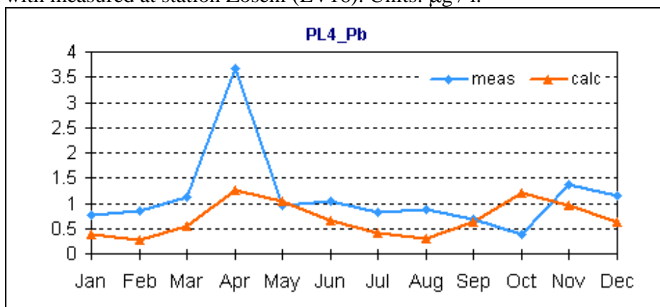
Figure 5.21. Comparison of calculated mean monthly lead concentrations in precipitation with measured at station Leba (PL04). Units: \mu\text{g} / \text{l} .
