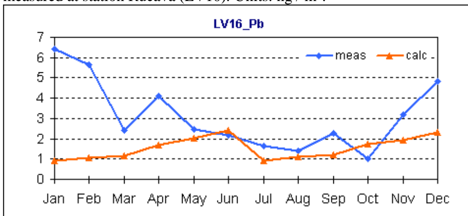
Figure 5.12. Comparison of calculated mean monthly lead concentrations in air with measured at station Zoseni (LV16). Units: \text{ng} / \text{m}^3 .
