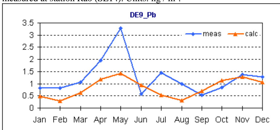
Figure 5.15. Comparison of calculated mean monthly lead concentrations in precipitation with measured at station Zingst (DE09). Units: \mu\text{g} / \text{l} .
