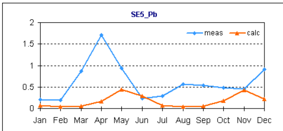
Figure 5.22. Comparison of calculated mean monthly lead concentrations in precipitation with measured at station Breckälen (SE05). Units: \mu\text{g} / \text{l} .
