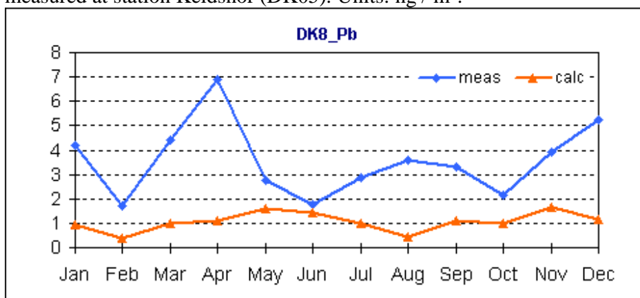
Figure 5.9. Comparison of calculated mean monthly lead concentrations in air with measured at station Anholt (DK08). Units: ng / m 3 .
