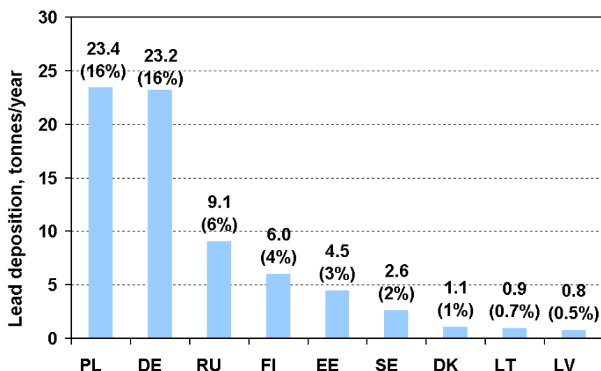
Figure 5.5. Contributions of HELCOM countries emissions from anthropogenic sources to total lead depositions to the Baltic Sea in 2002, tonnes/year
