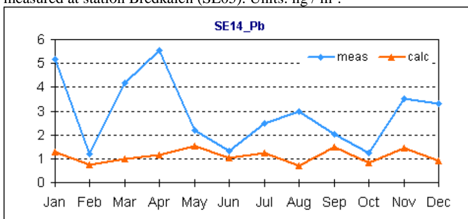
Figure 5.14. Comparison of calculated mean monthly lead concentrations in air with measured at station Råo (SE14). Units: \text{ng} / \text{m}^3 .
