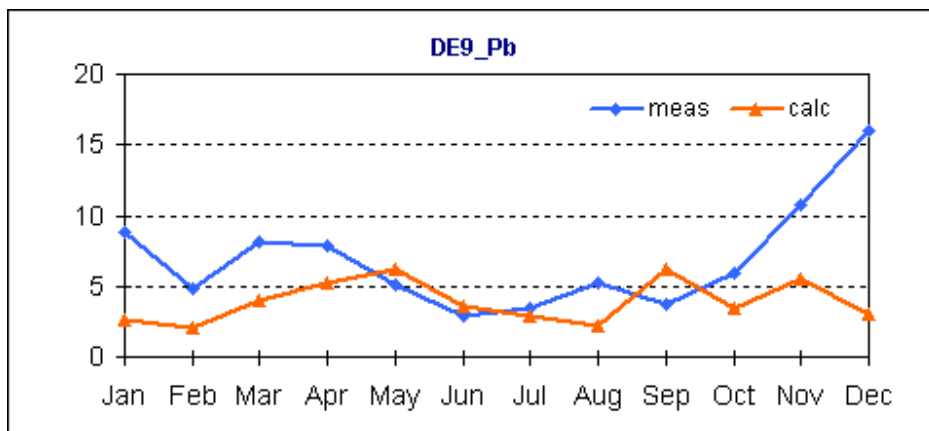
Figure 5.7. Comparison of calculated mean monthly lead concentrations in air with measured at station Zingst (DE09). Units: ng / m 3 .
