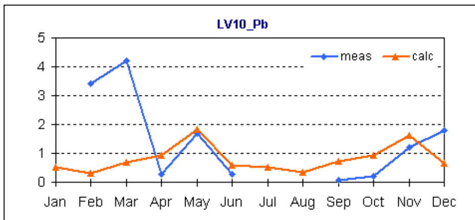
Figure 5.19. Comparison of calculated mean monthly lead concentrations in precipitation with measured at station Lahemaa (LV10). Units: \mu\text{g} / \text{l} .
