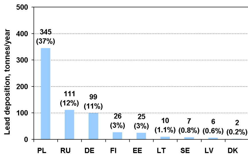
Figure 5.6. Contributions of HELCOM countries emissions from anthropogenic sources to total lead depositions to the Baltic Sea catchment area in 2002, tonnes/year
