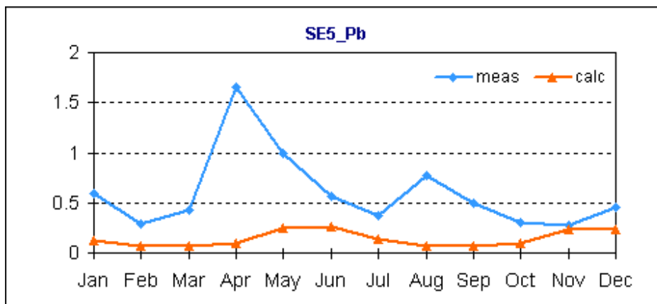
Figure 5.13. Comparison of calculated mean monthly lead concentrations in air with measured at station Bredkälén (SE05). Units: \text{ng} / \text{m}^3 .
