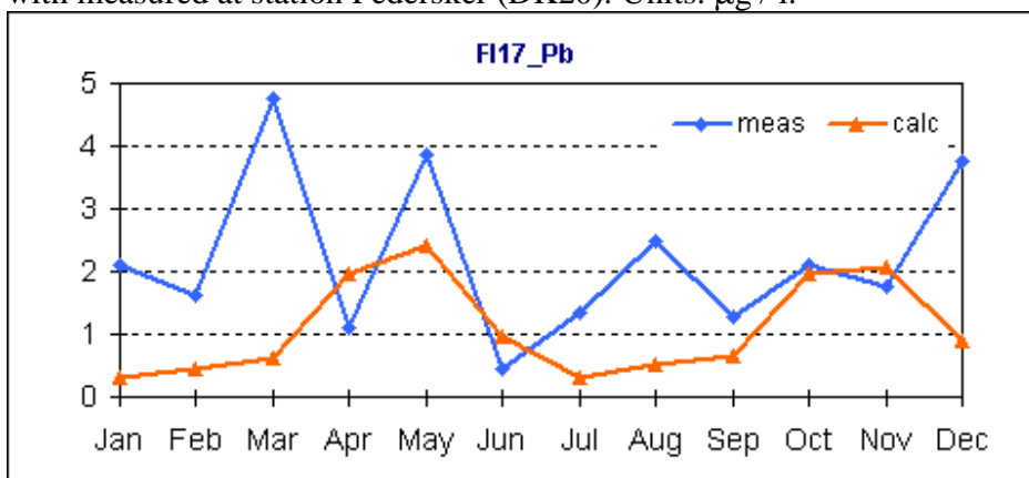
Figure 5.18. Comparison of calculated mean monthly lead concentrations in precipitation with measured at station Virolahti II (FI17). Units: \mu\text{g} / \text{l} .
