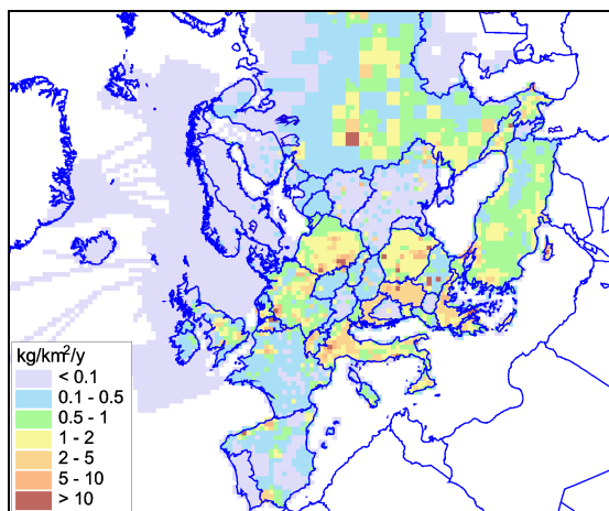
Figure 5.1. Spatial distribution of lead anthropogenic emission within the EMEP region in 2002 with resolution 50x50 km 2 . Units: kg/km 2 /year
