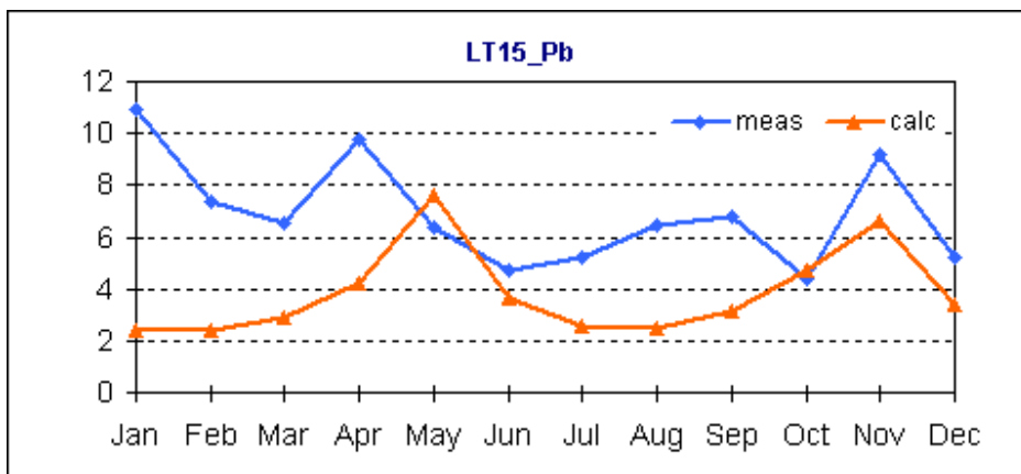
Figure 5.10. Comparison of calculated mean monthly lead concentrations in air with measured at station Preila (LT15). Units: \text{ng} / \text{m}^3 .
