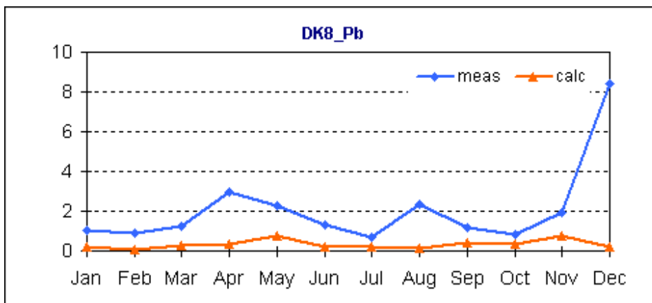
Figure 5.16. Comparison of calculated mean monthly lead concentrations in precipitation with measured at station Anholt (DK08). Units: \mu\text{g} / \text{l} .
