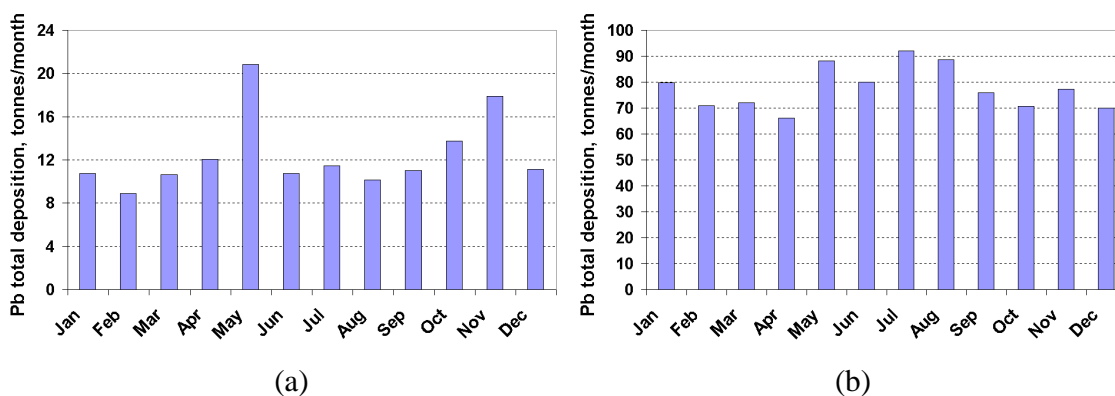
Figure 5.4. Monthly variations of lead total depositions to the Baltic Sea (a) and its catchment area (b) in 2002. Units: tonnes/month
