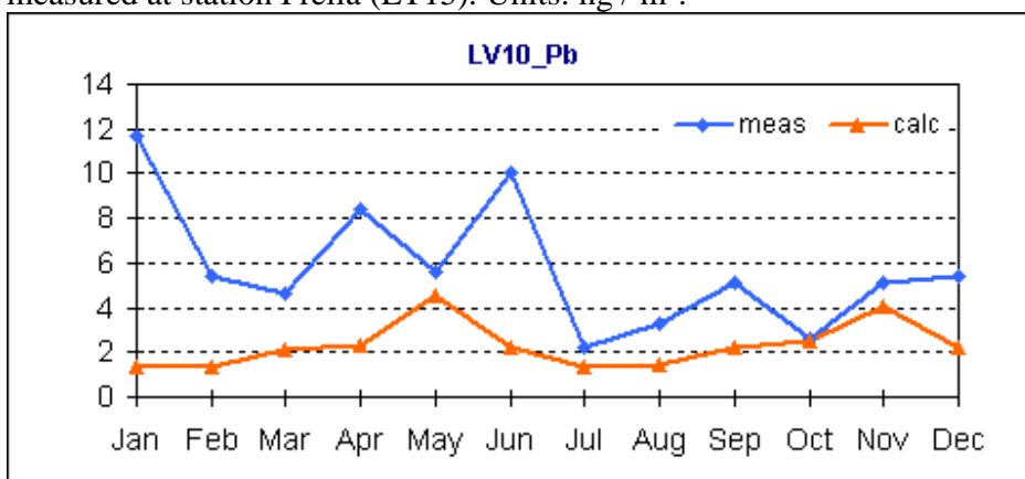
Figure 5.11. Comparison of calculated mean monthly lead concentrations in air with measured at station Rucava (LV10). Units: \text{ng} / \text{m}^3 .
